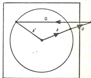
FIG. 17. Umklapp process.
