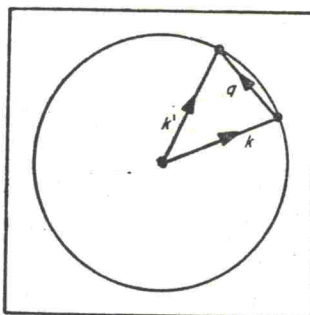
FIG. 16. Normal scattering process.
